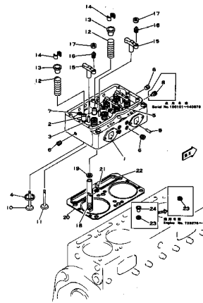
FIG. 1101 CYLINDER HEAD
