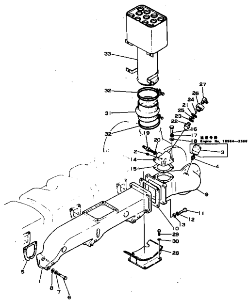
FIG. 111B AIR INTAKE MANIFOLD AND CONNECTION
