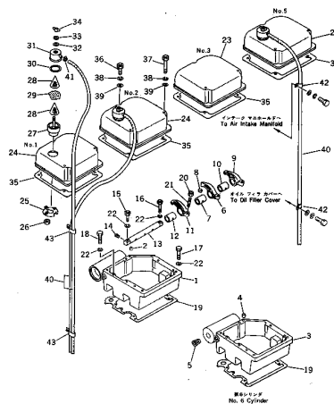
FIG. 107 ROCKER LEVER AND HOUSING
