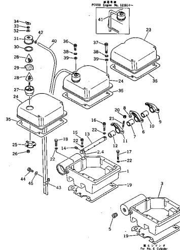
FIG.104 ROCKER LEVER AND HOUSING
