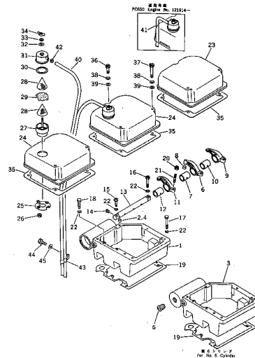
FIG. 104 ROCKER LEVER AND HOUSING
