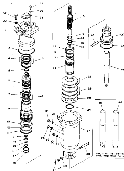
Fig. 101 IMPACTOR.
