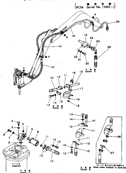
Fig.124 HYDRAURIC PIPING ATTACHMENT SIDE OUTLET
