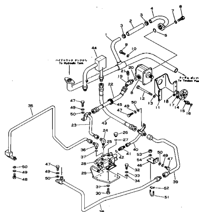
Fig. 142A HYDRAULIC PIPING, CHASSIS SIDE (PC04 Serial No. (2147~))
