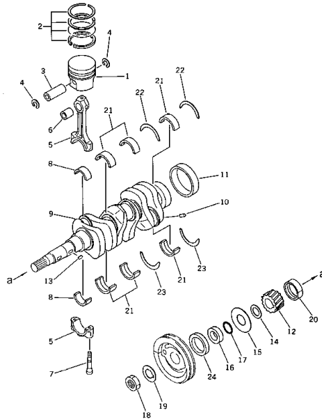
Fig. 111 PISTON AND CRANKSHAFT
