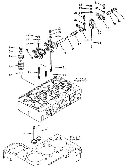
Fig. 107 ROCKER ARM, INLET AND EXHAUST VALVES
