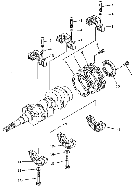
Fig. 105 MAIN BEARING CASE
