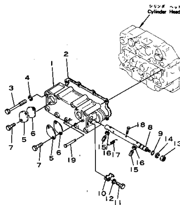
Fig. 106 CYLINDER HEAD COVER AND COMPRESSION RELEASE SHAFT
