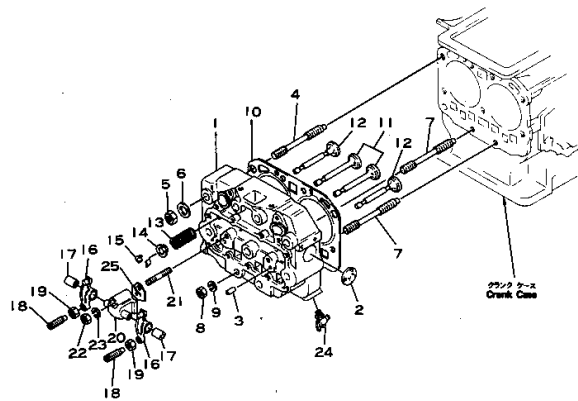
Fig. 105 CYLINDER HEAD AND VALVE
