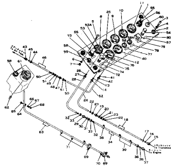
Fig.131 GAUGE AND PANEL (Serial No.0003~ )
