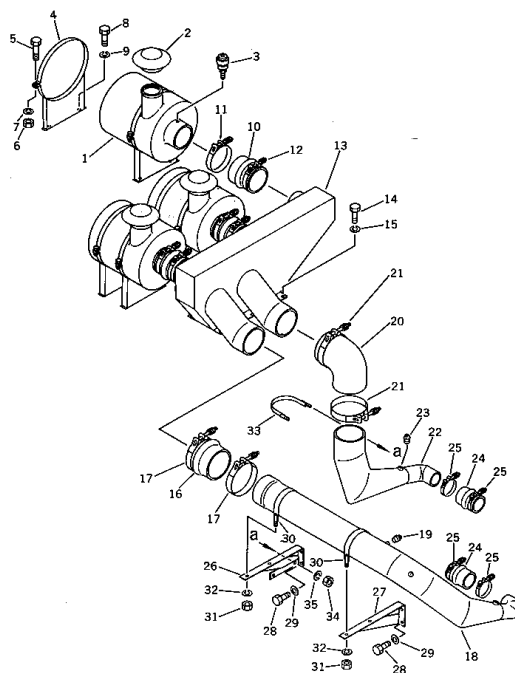
FIG. 1031 AIR INTAKE PIPING (FOR KOMATSU ENGINE)
