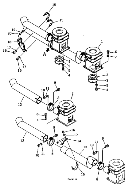
Fig. 118 EXHAUST SYSTEM (2/3) (Except U.K.)
