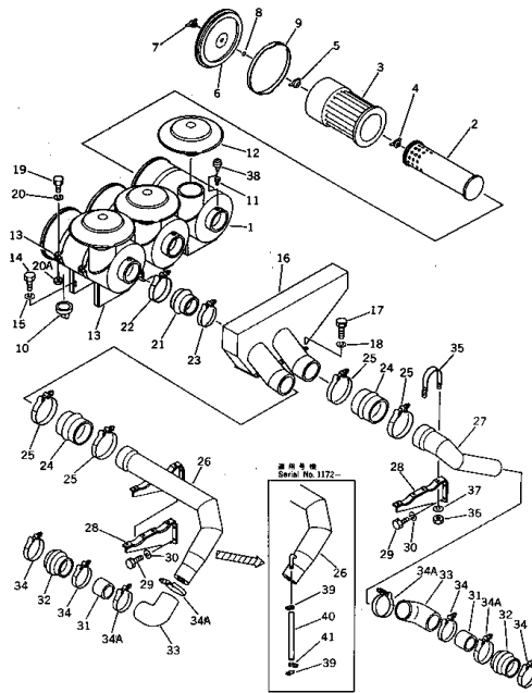
Fig. 115 AIR INTAKE SYSTEM
