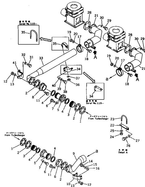
Fig. 117 EXHAUST SYSTEM (1/3)
