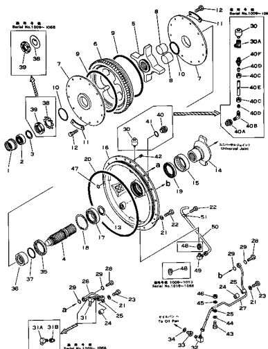
Fig. 103 ENGINE OUTPUT SHAFT (Serial No. 1002~1068)
