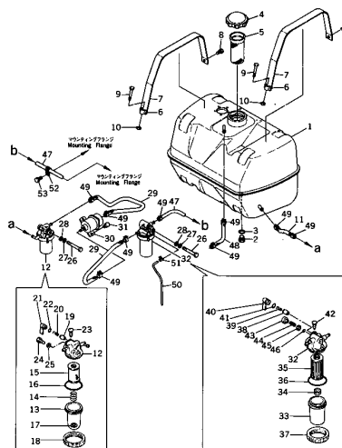
FIG. 1301 FUEL TANK AND PIPING
