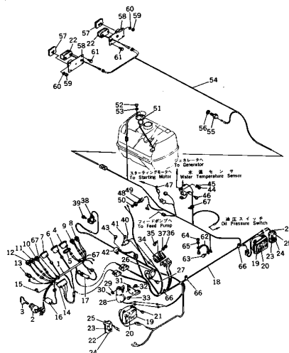
FIG. 1421 ELECTRICAL SYSTEM
