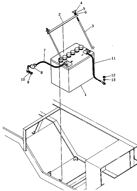
FIG. 1401 BATTERY AND CABLE
