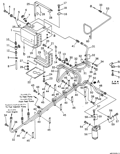
FIG. 1301 FUEL TANK AND PIPING
