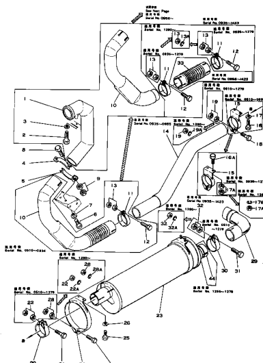
Fig. 1102 EXHAUST MUFFLER (1/2)
