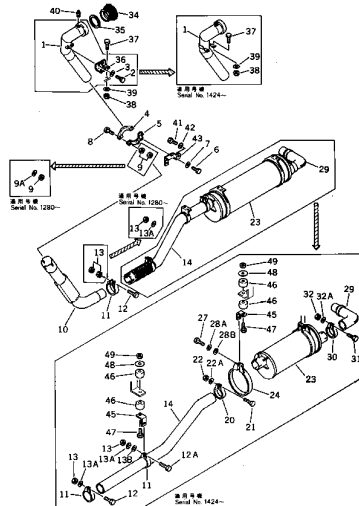
Fig. 1102A EXHAUST MUFFLER (3/2)
