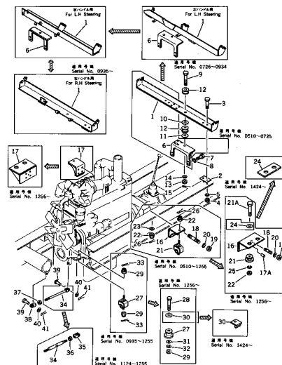
Fig. 1101 ENGINE AND TRANSMISSION MOUNTING PARTS
