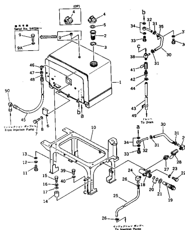
FIG. 142 FUEL TANK AND FUEL PIPING (GD605A SERIAL NO. 54001 -)
