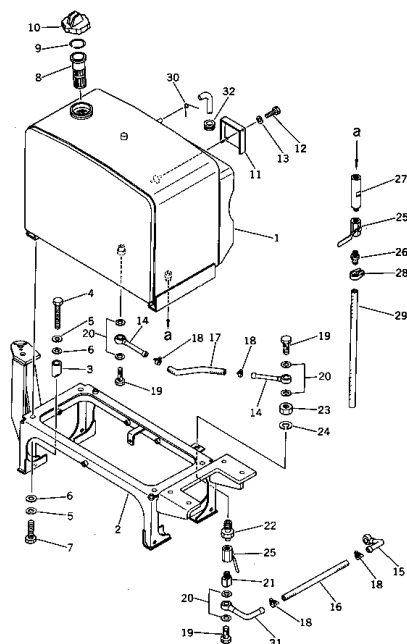
Fig. 141 FUEL TANK
