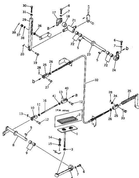
Fig. 121 FUEL CONTROL PEDAL LINKAGE
