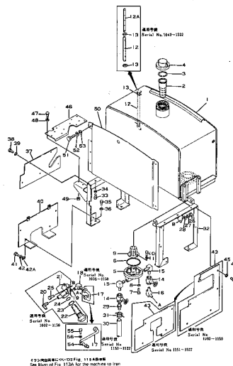
Fig. 113 FUEL TANK (Serial No. 1002~1522)
