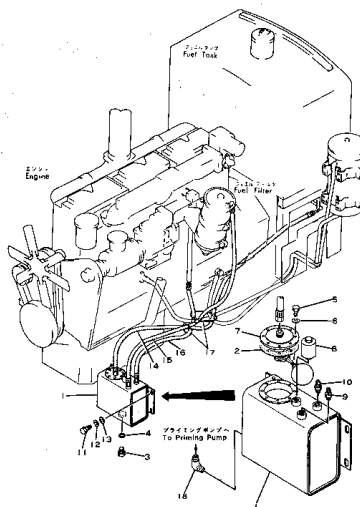
Fig.114 FUEL PIPING
