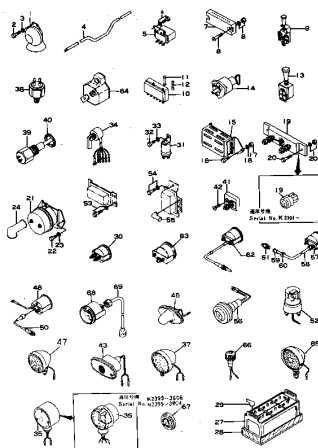
Fig. 131 B ELECTRICAL SYSTEM (1) (Serial No. 1585, 1618~)
