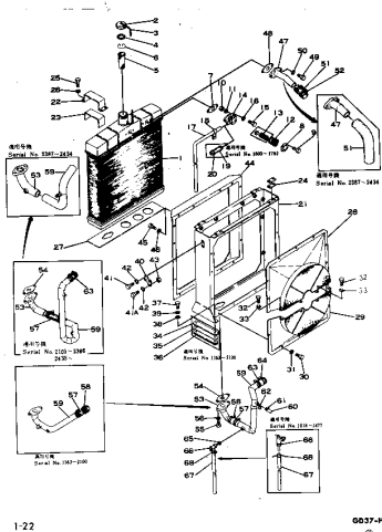
Fig. 115A RADIATOR (小松エンジン用散热器) (For Komatsu Engine Serial No. 1163~) (キムンエンジン用散热器) (For Cummins Engine Serial No. 1293~1617)
