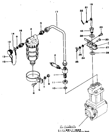
Fig. 113B COMPRESSOR AIR CLEANER AND PIPING (For Komatsu Engine Serial No. 1328~) (OPTIONAL PART)
