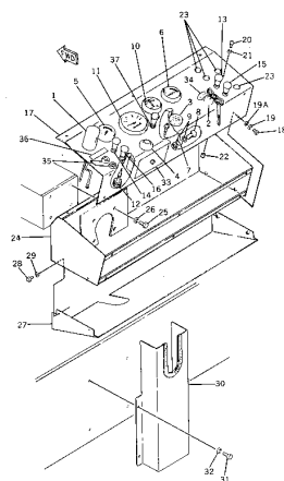
Fig. 133B INSTRUMENT PANEL (Serial No. 3152~)
