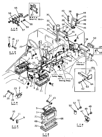
Fig. 132C ELECTRICAL SYSTEM REAR (Serial No. 4001~)
