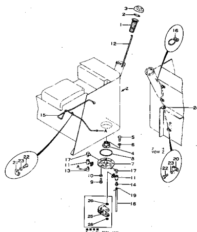
Fig. 112A FUEL TANK RELATED PARTS (Serial No. 1336~)
