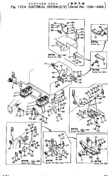
Fig. 132A ELECTRICAL SYSTEM (2/2) (Serial No. 1336~4000)
