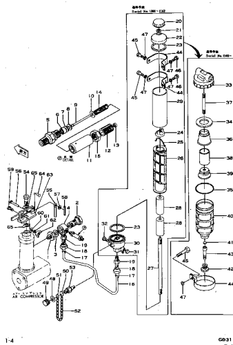
Fig. 105 AIR COMPRESSOR RELATED PARTS (Serial No. 1003~1335)
