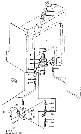
Fig. 111A FUEL TANK RELATED PARTS (適用号機 (Serial No. 801~))
