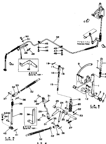
Fig. 101 ACCELERATOR LEVER
