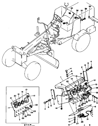
Fig. 131 INSTRUMENT PANEL (Serial No. 1003~)
