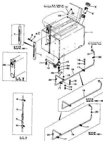
Fig. 111 FUEL TANK AND PIPING
