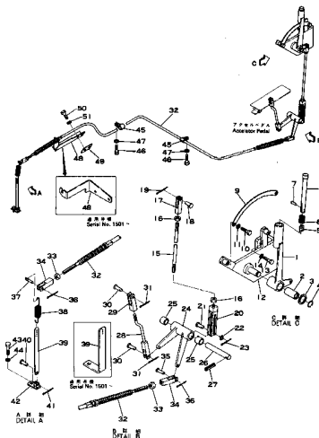
Fig. 101 ACCELERATOR LEVER
