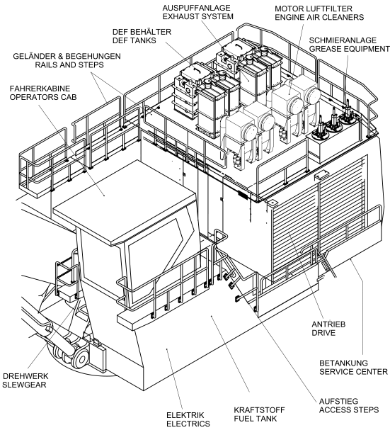
Oberwagen Superstructure
