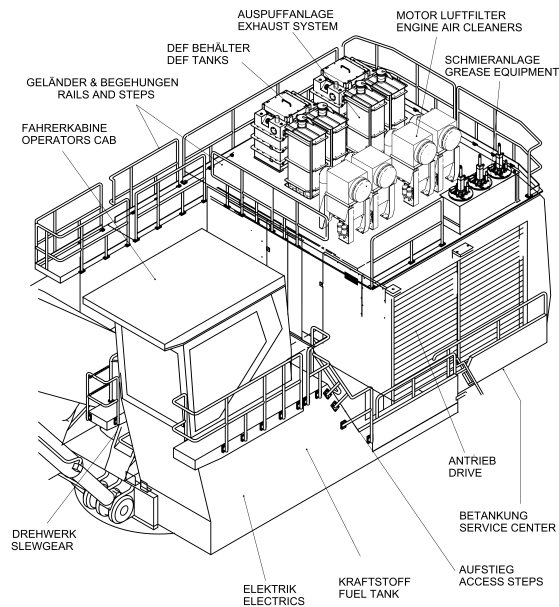
Oberwagen Superstructure
