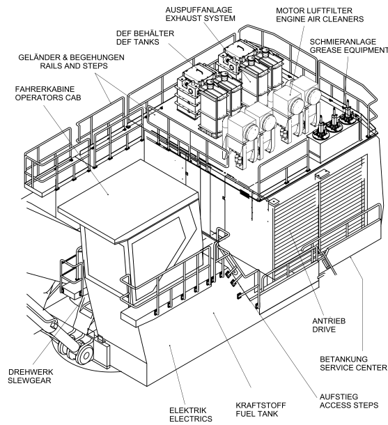
Oberwagen Superstructure
