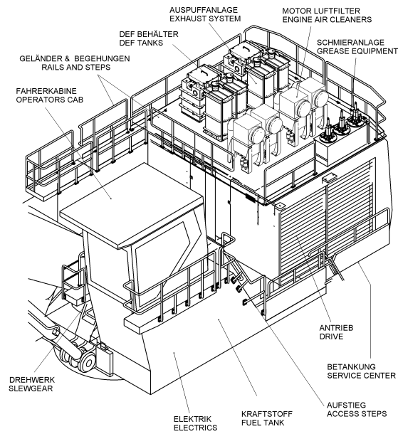
Oberwagen Superstructure
