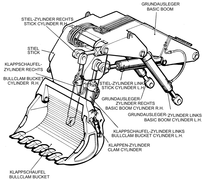
Klappschaufel-Einrichtung (KSE) Bullclam Bucket Equipment (BBE)
