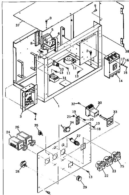
FIG. 2201 CONTROL BOX ASS'Y (EG85BS SERIAL NO. 4501- )
