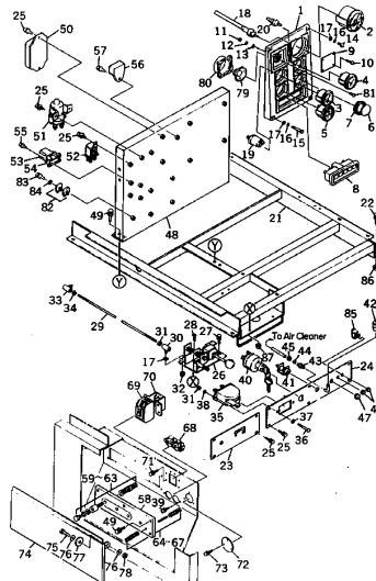
FIG. 4201 ENGINE OPERATING PANEL ASS'Y (EG85BS SERIAL NO. 4501- )
