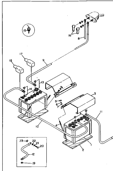
FIG. 5201 BATTERY ASS'Y (EG85BS SERIAL NO. 4501-)
