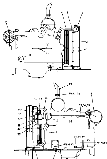
FIG. 3001 RADIATOR ASS'Y (EG85 SERIAL NO. 4001-) (EG85B SERIAL NO. 4001-)
