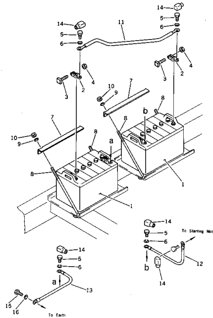
Fig. 141 BATTERY AND CABLE (EG80 Serial No. 1001~)
