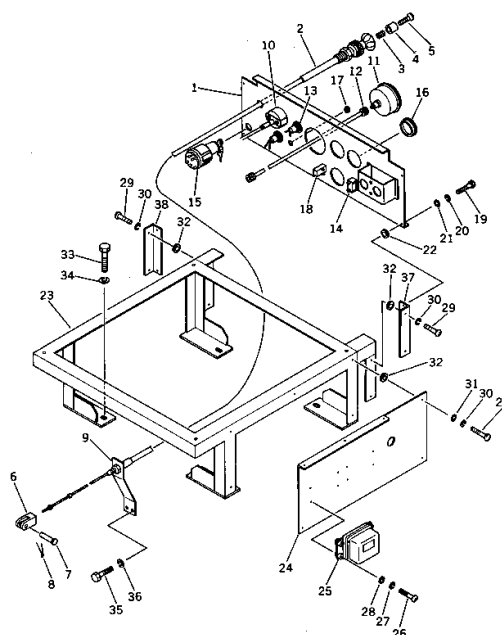
Fig. 145 ENGINE INSTRUMENT PANEL
