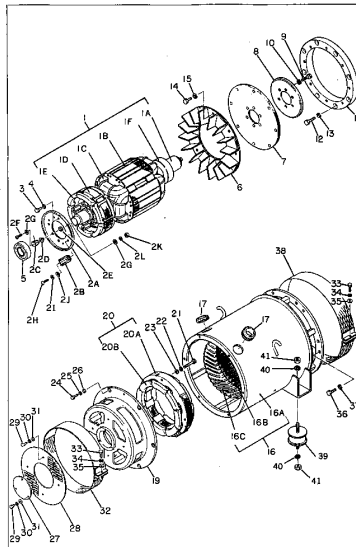
FIG. 1201 GENERATOR ASS'Y (EG60BS)
