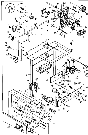
FIG. 4201 ENGINE OPERATING PANEL ASS'Y (EG60BS)
