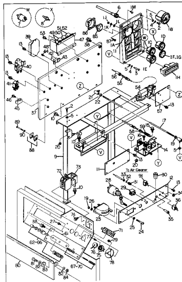
FIG. 4211 ENGINE OPERATING PANEL ASS'Y (WITH AUTOMATIC IDLING) (EG60BS)
