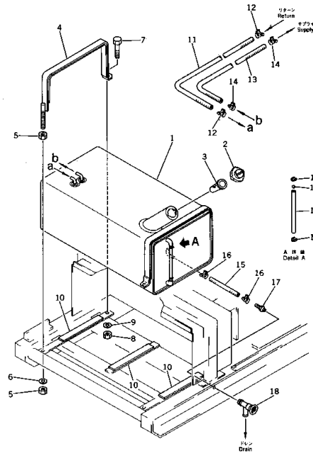
Fig. 132 FUEL TANK (EG55S Serial No. 1001~)
