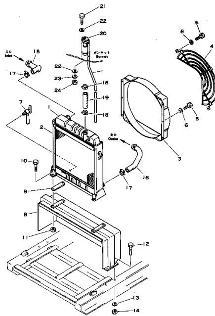
Fig. 121A RADIATOR AND MOUNTING (EG55 Serial No. 1132~)
