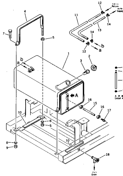
Fig. 131 FUEL TANK (EG55 Serial No. 1001~)
