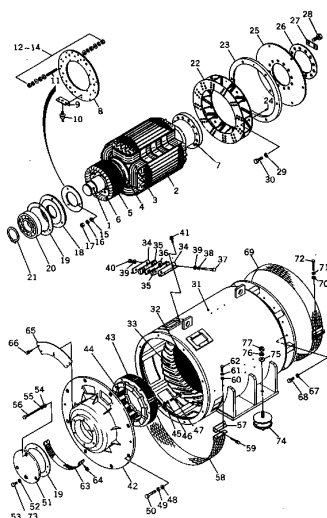
FIG. 1201 GENERATOR ASS'Y
