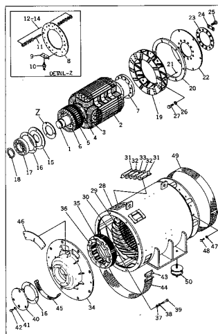
FIG. 1001 GENERATOR ASS'Y
