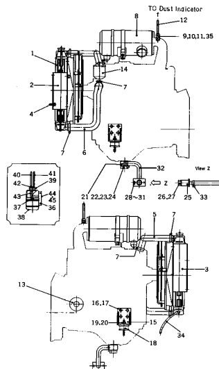
FIG. 3201 RADIATOR ASS'Y (EG40BS)
