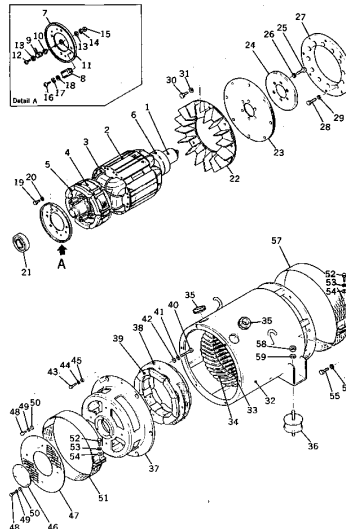
FIG. 1201 GENERATOR ASS'Y (EG40BS)
