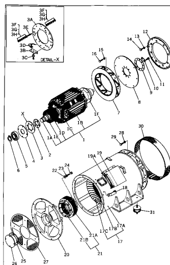
Fig. 1001 GENERATOR ASS'Y (EG350,350B)
