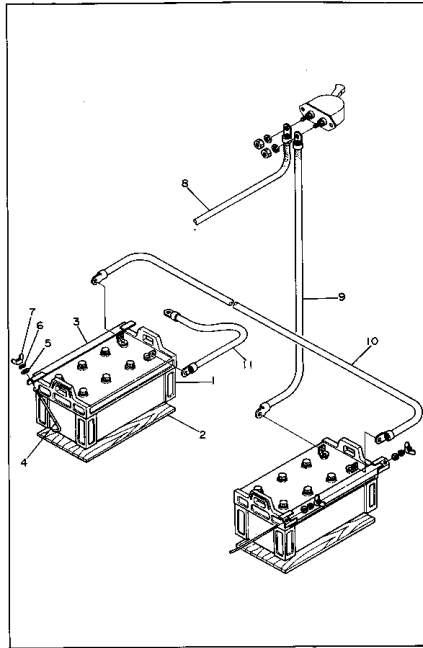
Fig. 5001 BATTERY ASS'Y (EG350,350B)
