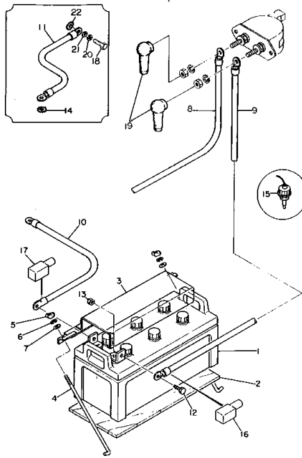
FIG. 5201 BATTERY ASS'Y (EG33BS)
