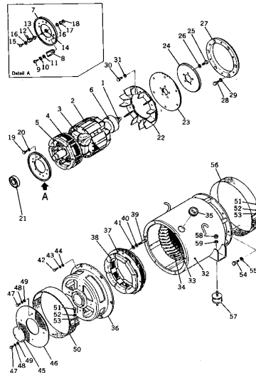
FIG. 1201 GENERATOR ASS'Y (EG33BS)
