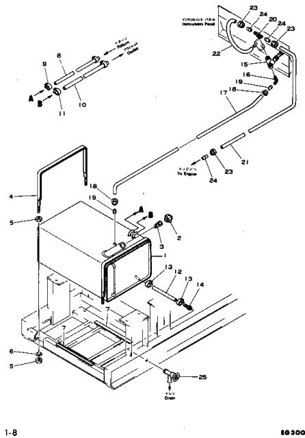
Fig. 131 FUEL TANK
