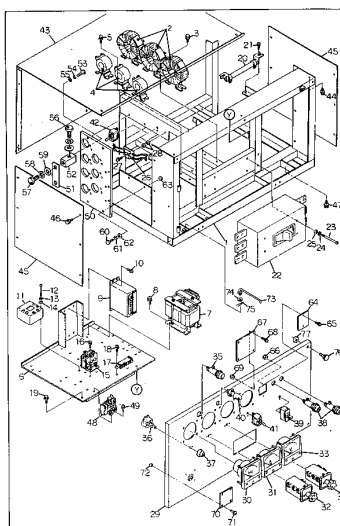
Fig. 2201 CONTROL BOX ASS'Y (EG275BS)
