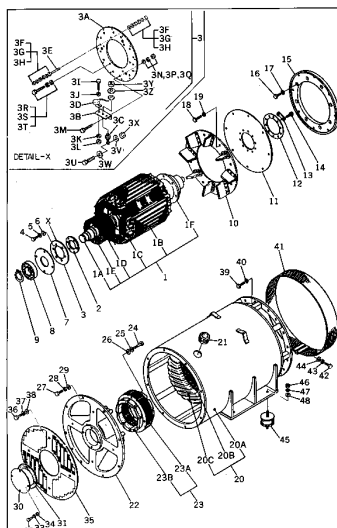
Fig. 1201 GENERATOR ASS'Y (EG275BS)
