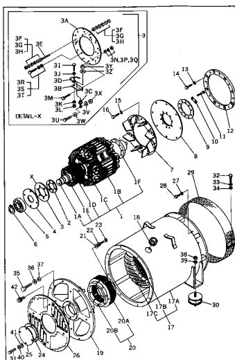
Fig. 1201 GENERATOR ASS'Y (EG220BS)
