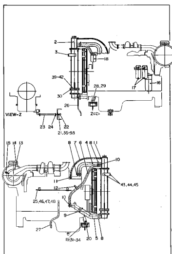
Fig. 3201 ラジエータ 組立 (EG220BS) RADIATOR ASS'Y (EG220BS)
