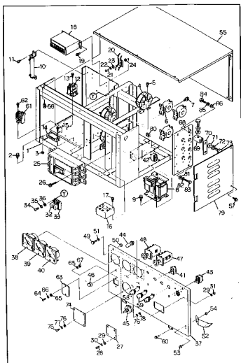
Fig. 2201 CONTROL BOX ASS'Y (EG220BS)
