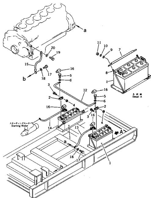
Fig. 141 BATTERY AND CABLE (EG200 Serial No. 3001~)
