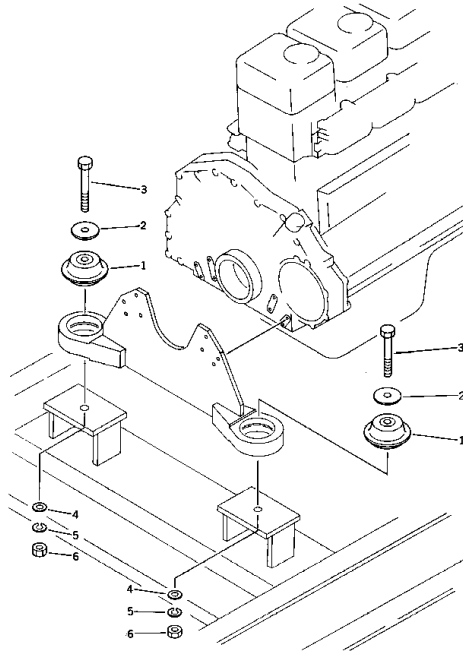
Fig. 101 ENGINE MOUNTING PARTS
