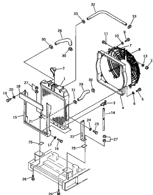
Fig. 121 RADIATOR AND MOUNTING (EG200 Serial No. 3001- )
