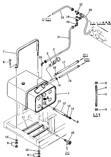
Fig. 1141 FUEL TANK \EG175 Serial No. 2001~ /
