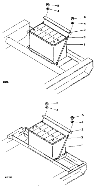
Fig. 141 BATTERY
