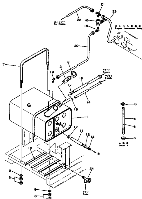
Fig. 131 FUEL TANK
