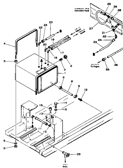
Fig. 131 FUEL TANK
