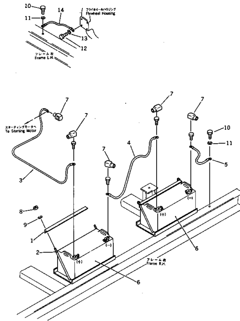
Fig. 142 BATTERY AND CABLE (EG125S Serial No. 1001~)
